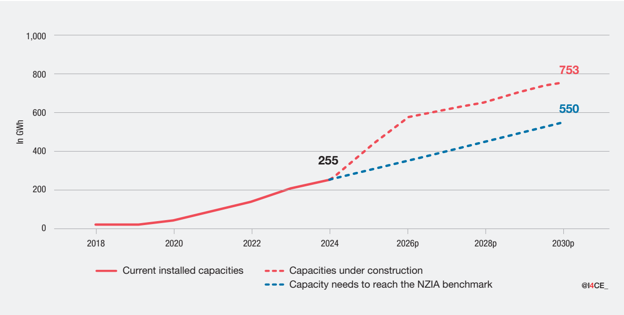
FIGURE 33. THE EU IS ON TRACK TO REACH THE 550 GWH BENCHMARK FOR BATTERY MANUFACTURING SET IN THE NZIA, CONSIDERING THE CAPACITIES THAT ARE TODAY UNDER CONSTRUCTION
