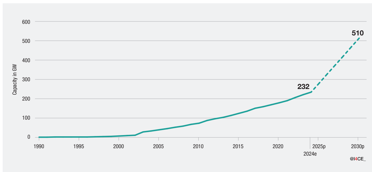
FIGURE 10. TO MEET EU 2030 WIND POWER TARGETS, INSTALLED CAPACITIES WILL NEED TO BE MULTIPLIED BY 2.2 BETWEEN 2025 AND 2030
