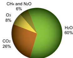
Share of the main greenhouse gases in the reflection of radiation towards the surface (in \text{W/m}^2 )
